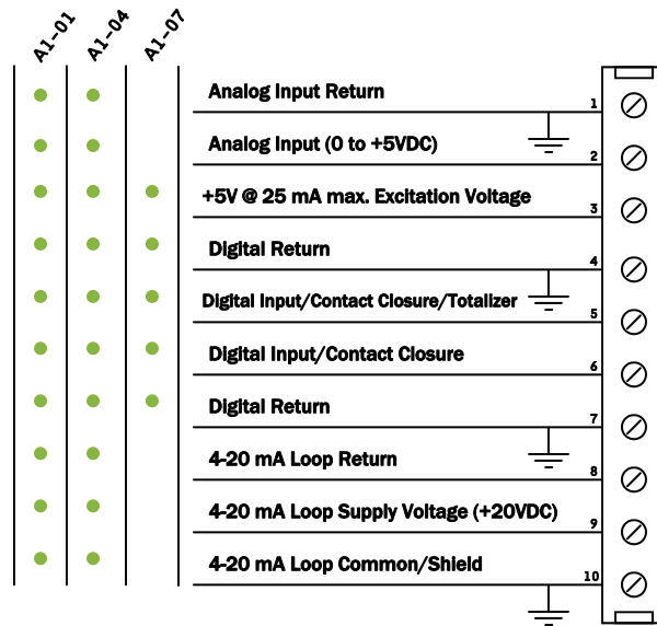
Pin 1 Pin 10
